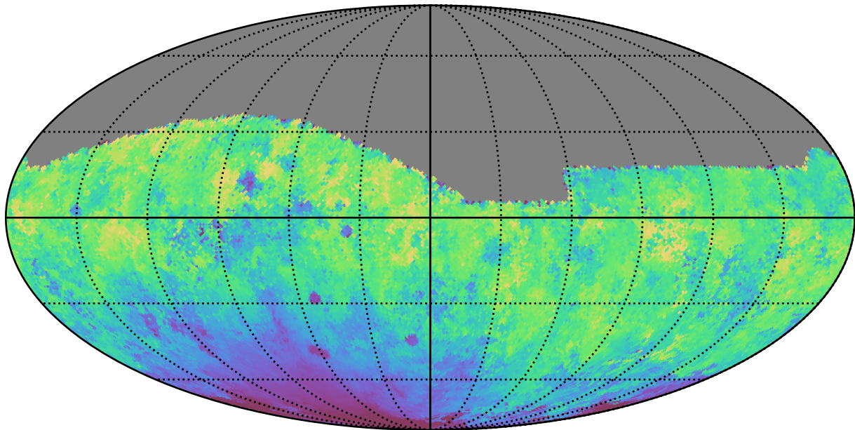
noroll_mjdp270_v3.4_10yrs All sky g band: Median moonDistance
