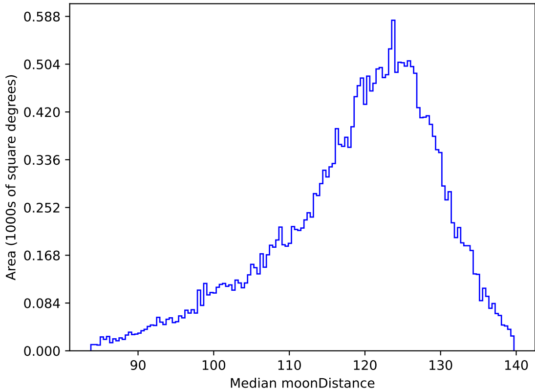
noroll_mjdp270_v3.4_10yrs All sky g band: Median moonDistance
