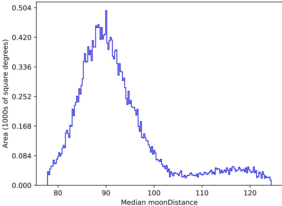
noroll_mjdp270_v3.4_10yrs All sky all bands: Median moonDistance
