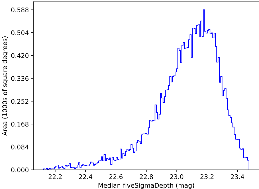
noroll_mjdp270_v3.4_10yrs Yr 1 z band: Median fiveSigmaDepth
