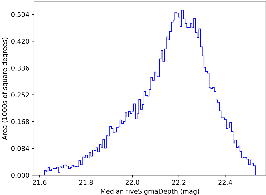
noroll_mjdp270_v3.4_10yrs Yr 1 y band: Median fiveSigmaDepth
