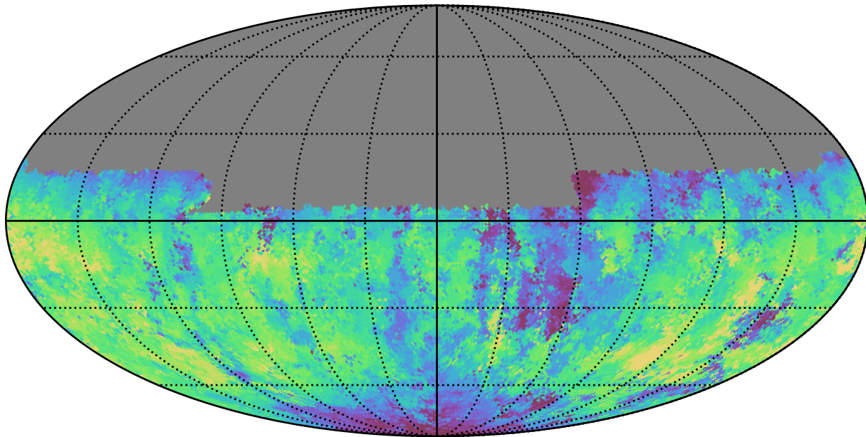
noroll_mjdp270_v3.4_10yrs Yr 1 u band: Median fiveSigmaDepth
