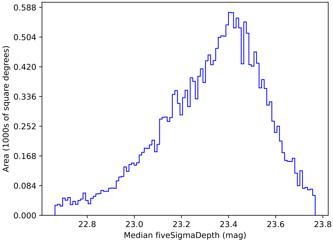
noroll_mjdp270_v3.4_10yrs Yr 1 u band: Median fiveSigmaDepth
