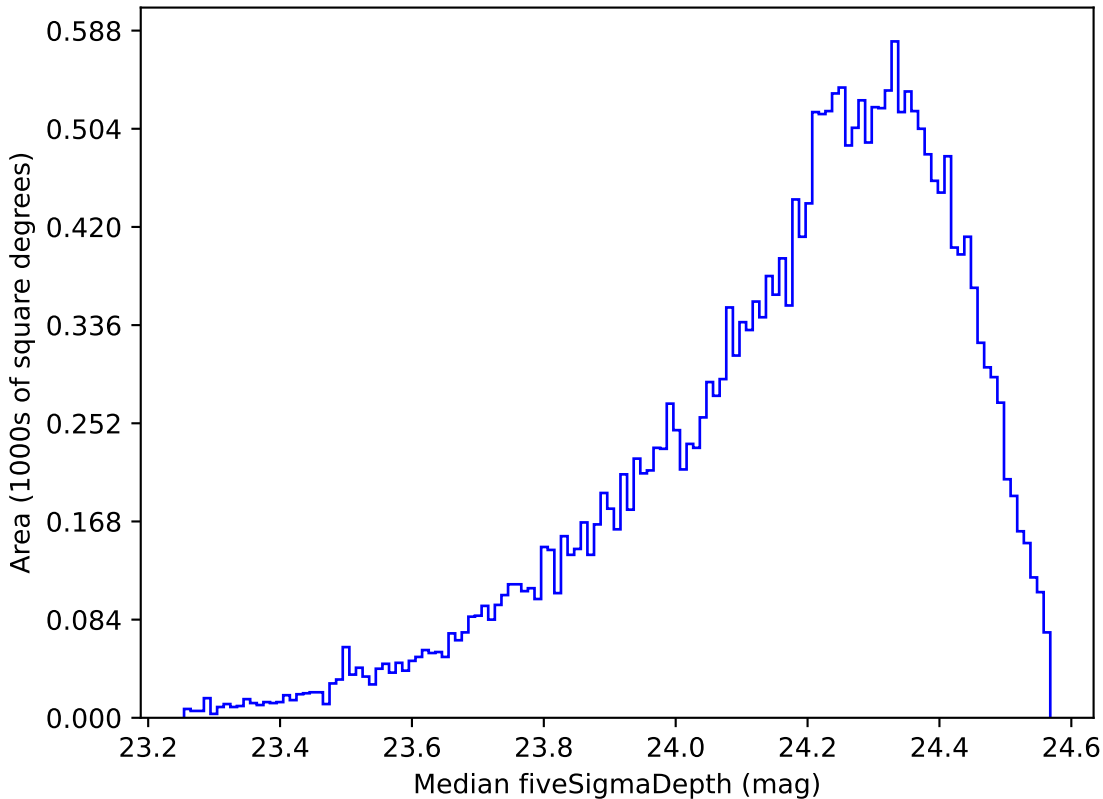
noroll_mjdp270_v3.4_10yrs Yr 1 r band: Median fiveSigmaDepth
