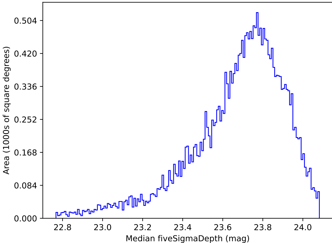
noroll_mjdp270_v3.4_10yrs Yr 1 i band: Median fiveSigmaDepth
