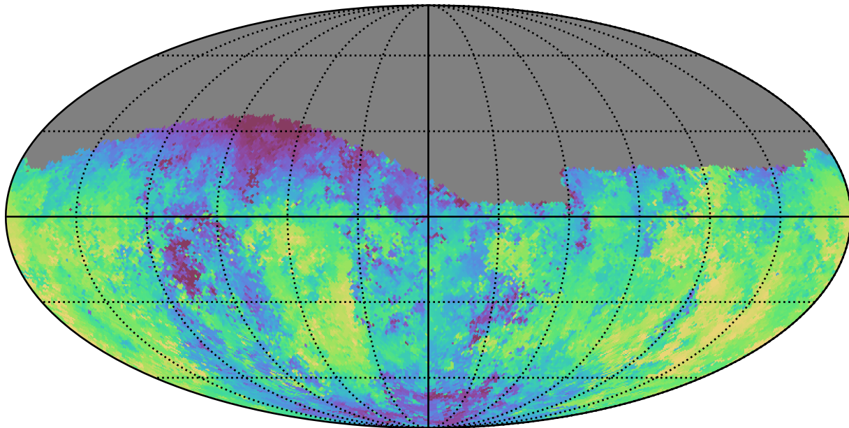
noroll_mjdp270_v3.4_10yrs Yr 1 g band: Median fiveSigmaDepth
