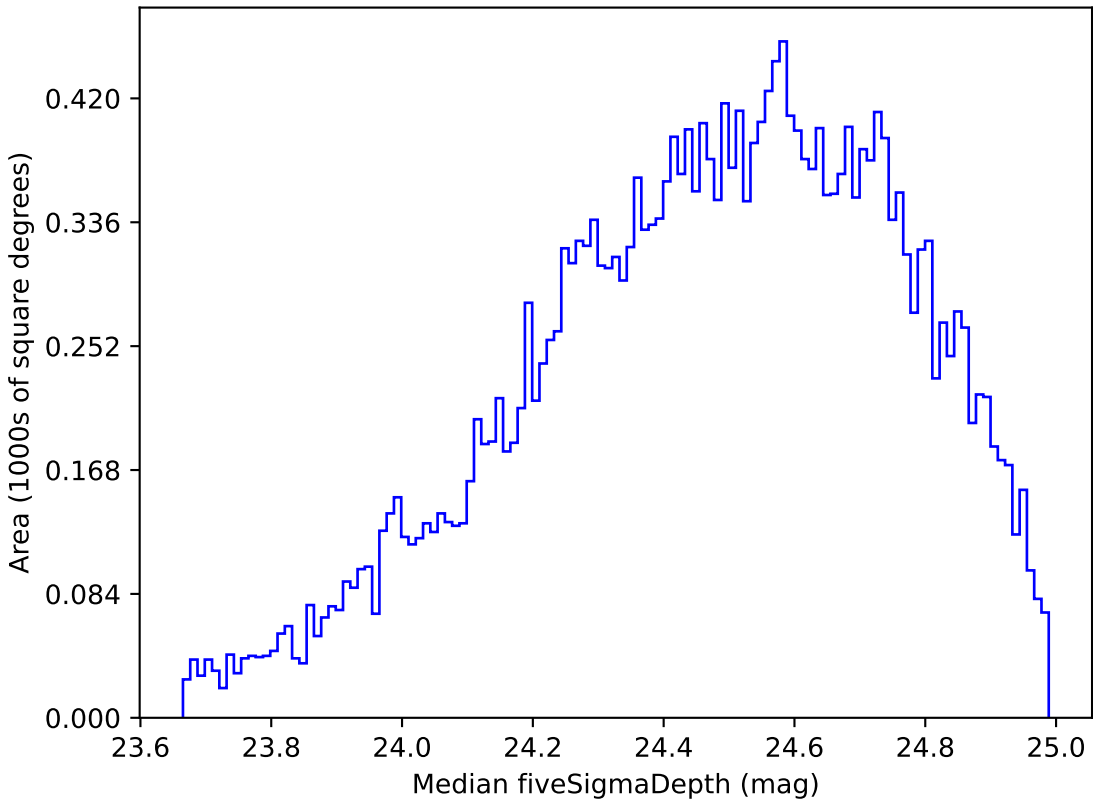
noroll_mjdp270_v3.4_10yrs Yr 1 g band: Median fiveSigmaDepth
