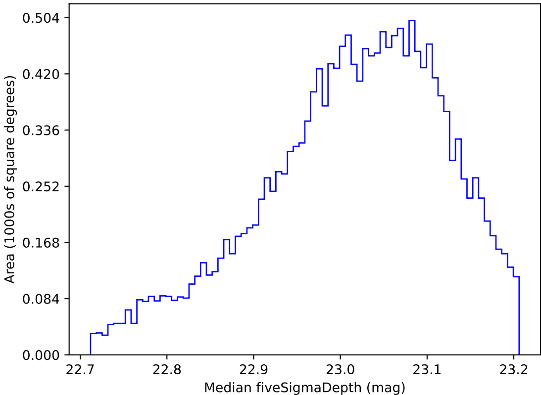
noroll_mjdp270_v3.4_10yrs WFD z band: Median fiveSigmaDepth
