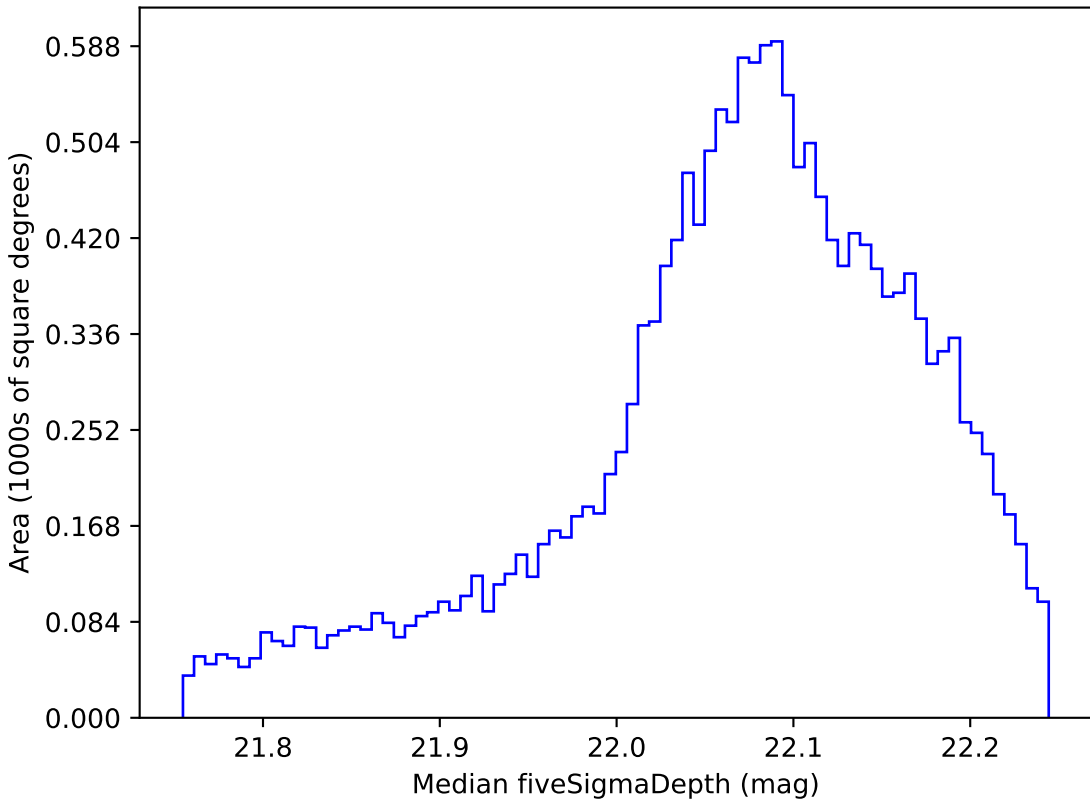
noroll_mjdp270_v3.4_10yrs WFD y band: Median fiveSigmaDepth
