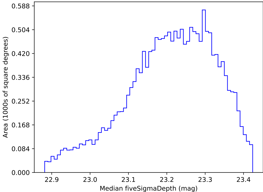
noroll_mjdp270_v3.4_10yrs WFD u band: Median fiveSigmaDepth
