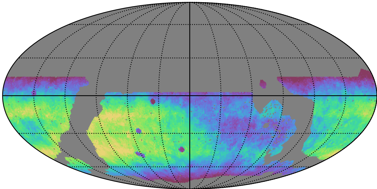
noroll_mjdp270_v3.4_10yrs WFD r band: Median fiveSigmaDepth
