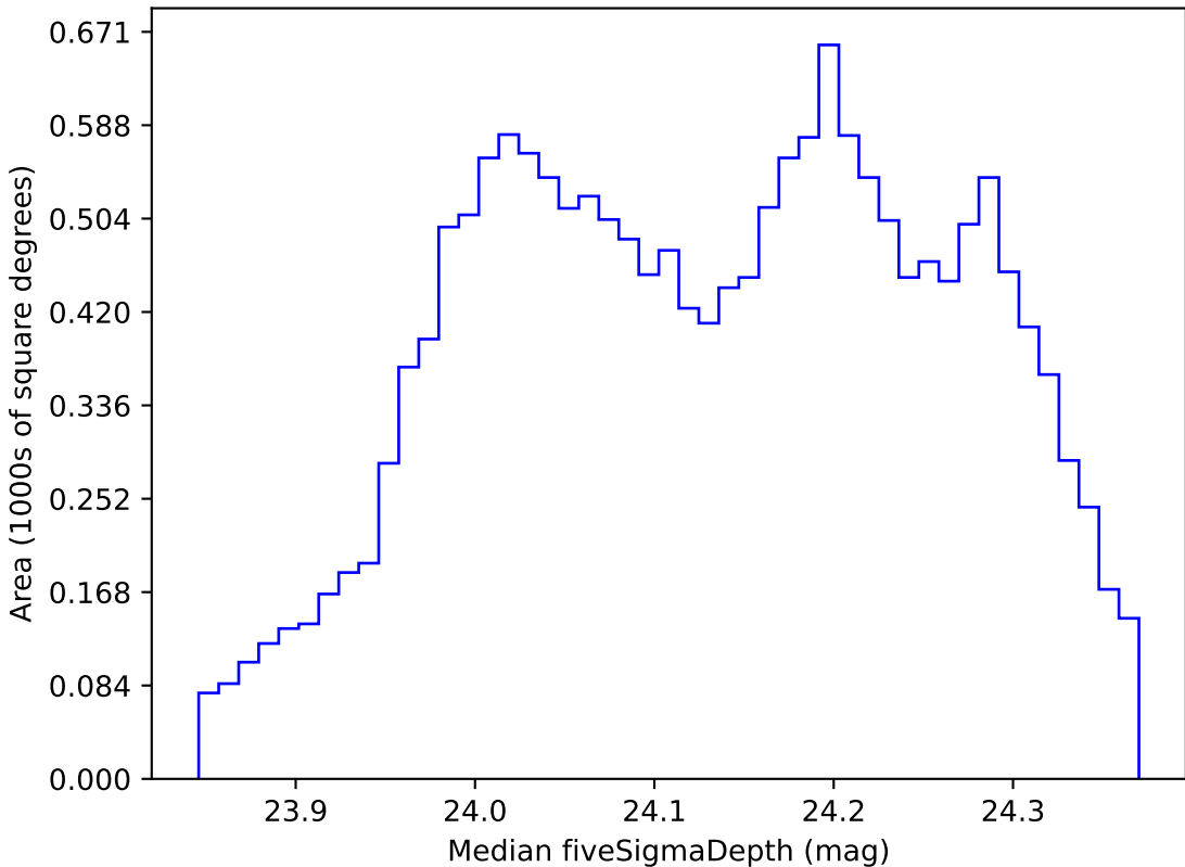
noroll_mjdp270_v3.4_10yrs WFD r band: Median fiveSigmaDepth
