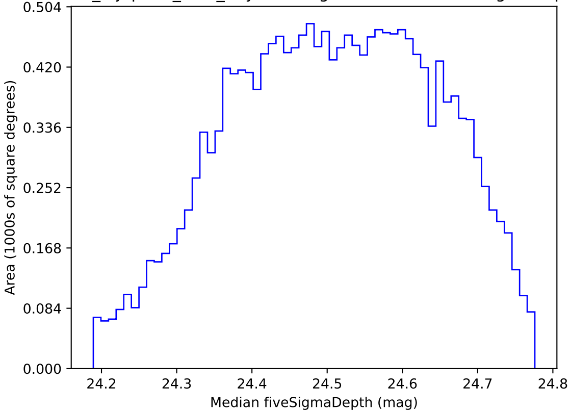
noroll_mjdp270_v3.4_10yrs WFD g band: Median fiveSigmaDepth
