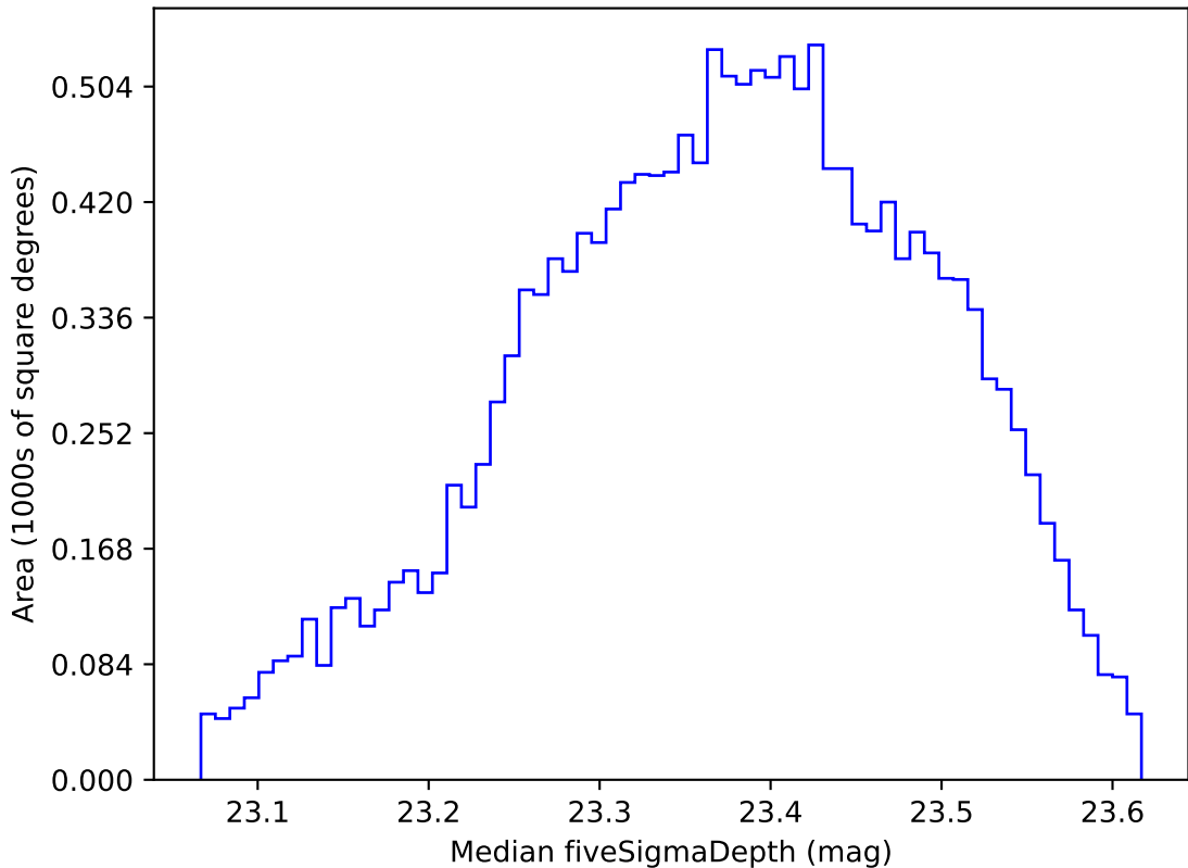
noroll_mjdp270_v3.4_10yrs WFD all bands: Median fiveSigmaDepth
