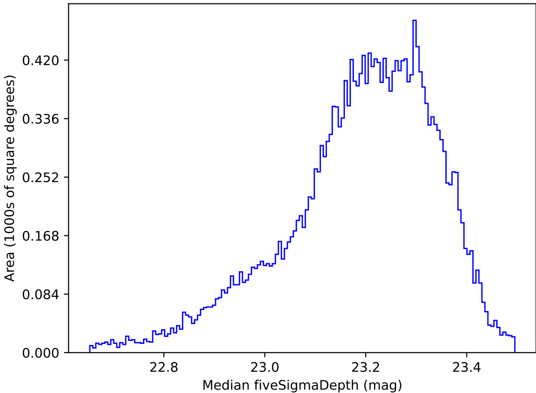
noroll_mjdp270_v3.4_10yrs All sky u band: Median fiveSigmaDepth
