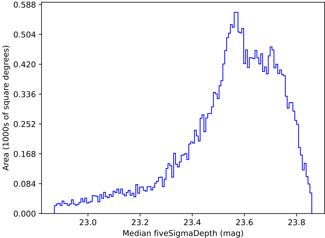
noroll_mjdp270_v3.4_10yrs All sky i band: Median fiveSigmaDepth
