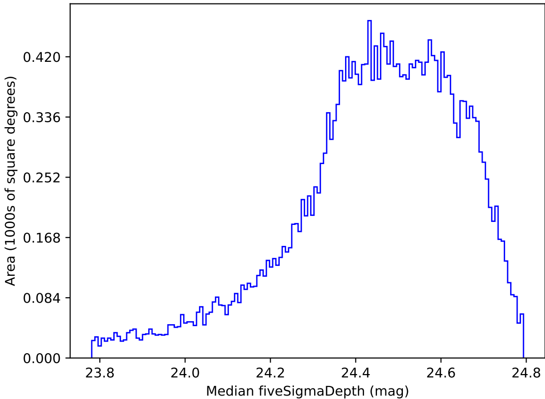
noroll_mjdp270_v3.4_10yrs All sky g band: Median fiveSigmaDepth
