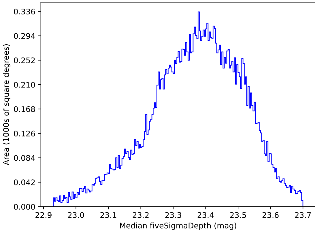
noroll_mjdp270_v3.4_10yrs All sky all bands: Median fiveSigmaDepth
