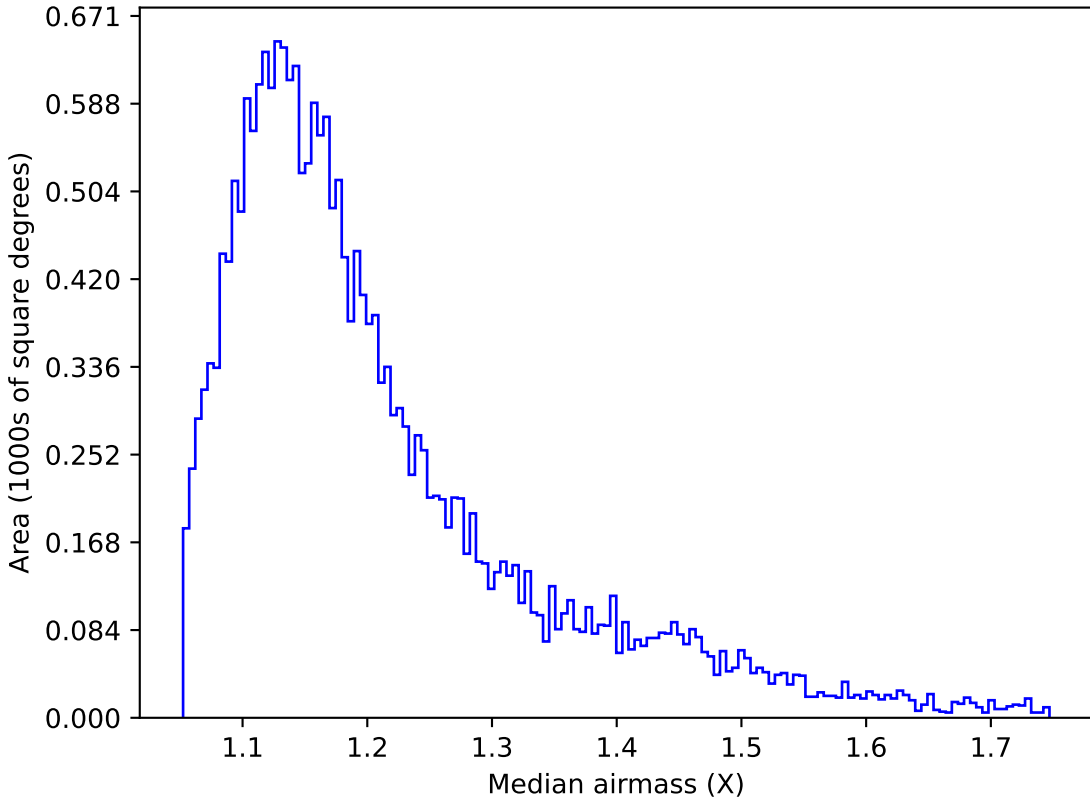
noroll_mjdp270_v3.4_10yrs Yr 1 u band: Median airmass
