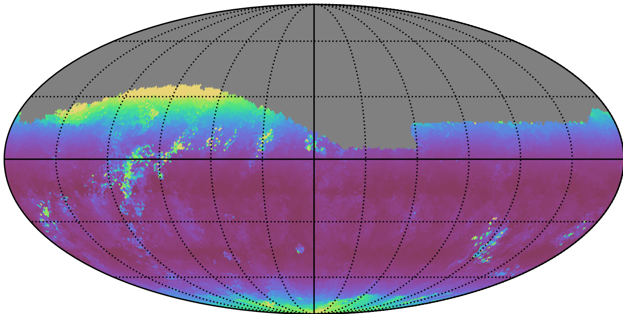
noroll_mjdp270_v3.4_10yrs Yr 1 r band: Median airmass
