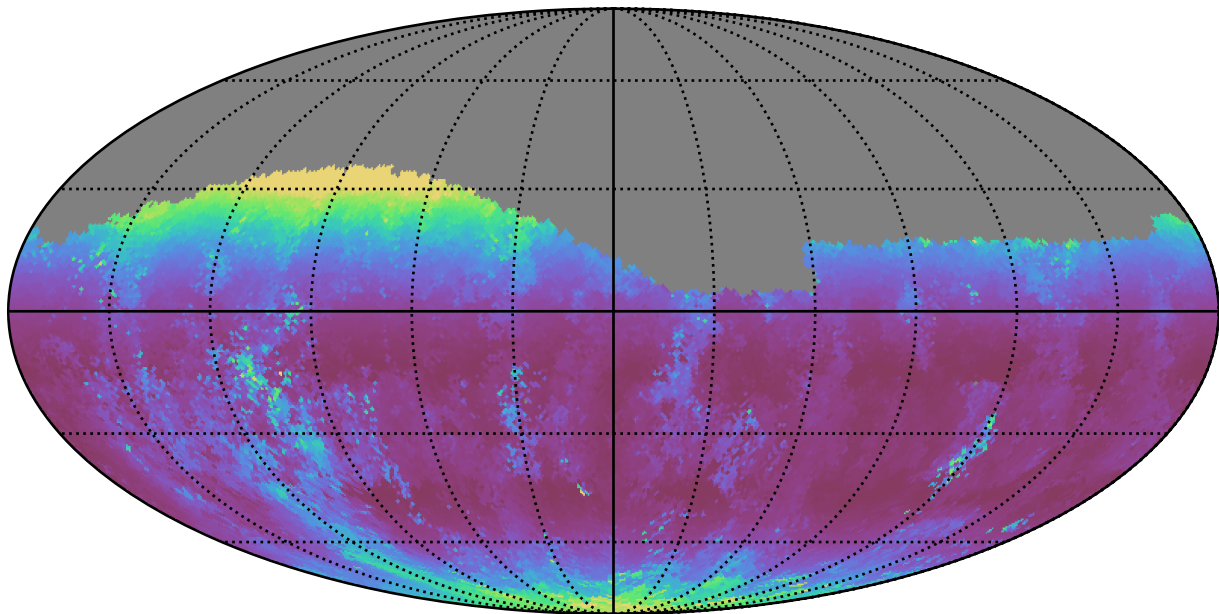
noroll_mjdp270_v3.4_10yrs Yr 1 g band: Median airmass
