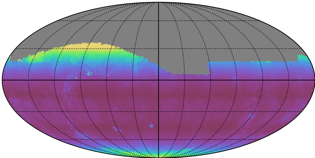
noroll_mjdp270_v3.4_10yrs Yr 1 all bands: Median airmass
