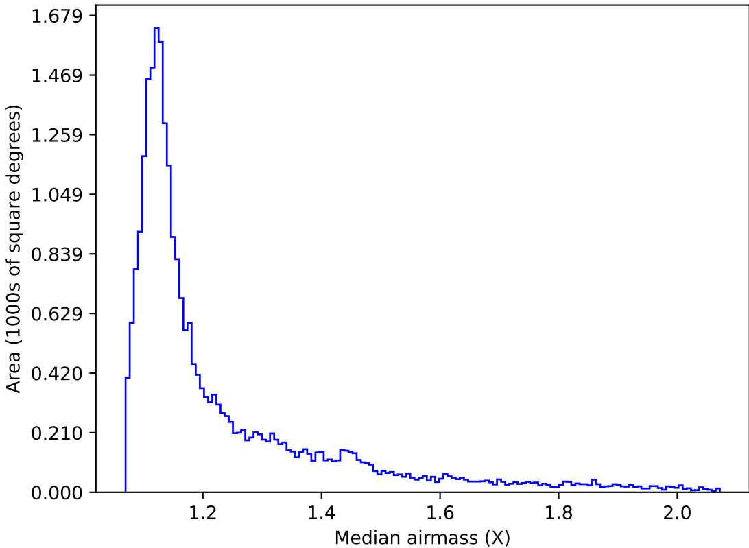
noroll_mjdp270_v3.4_10yrs Yr 1 all bands: Median airmass
