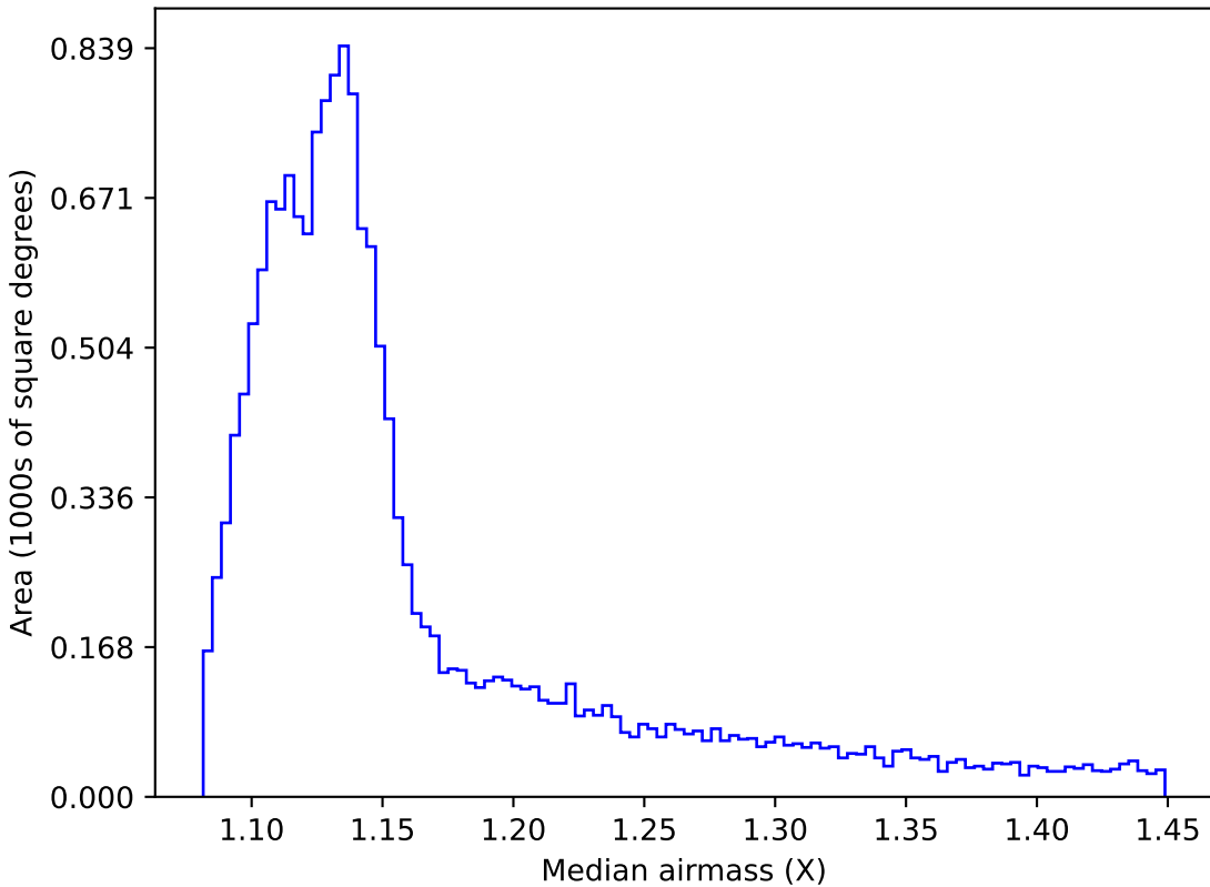
noroll_mjdp270_v3.4_10yrs WFD z band: Median airmass
