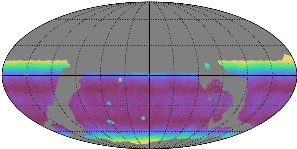
noroll_mjdp270_v3.4_10yrs WFD y band: Median airmass
