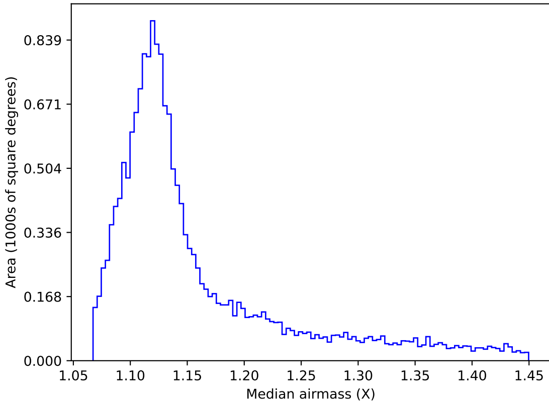
noroll_mjdp270_v3.4_10yrs WFD u band: Median airmass
