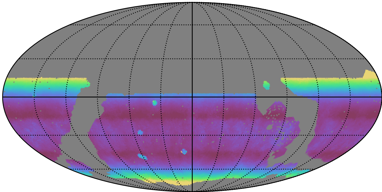
noroll_mjdp270_v3.4_10yrs WFD r band: Median airmass
