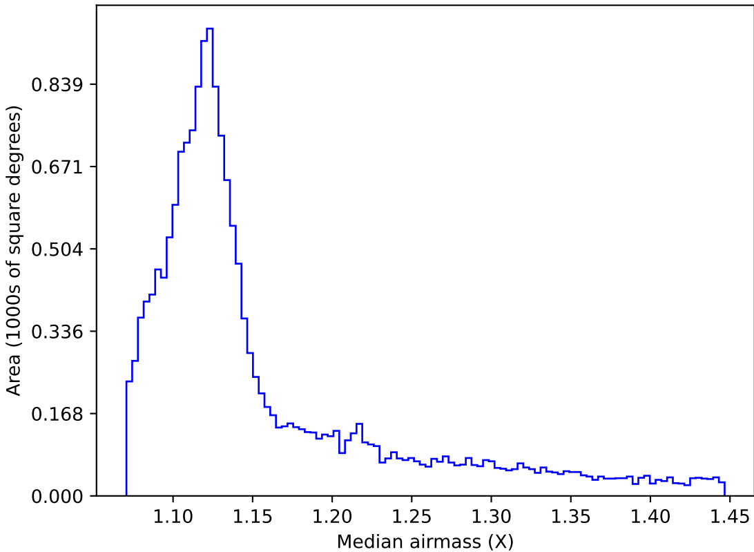
noroll_mjdp270_v3.4_10yrs WFD r band: Median airmass
