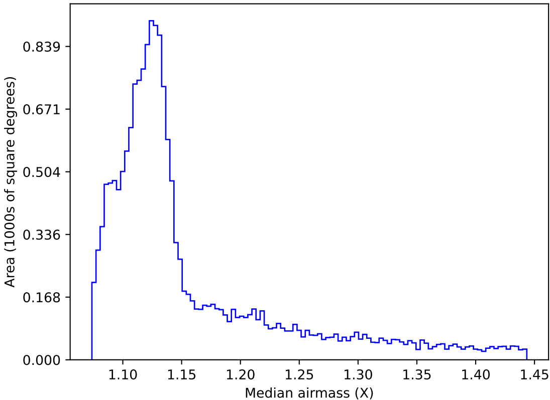
noroll_mjdp270_v3.4_10yrs WFD i band: Median airmass
