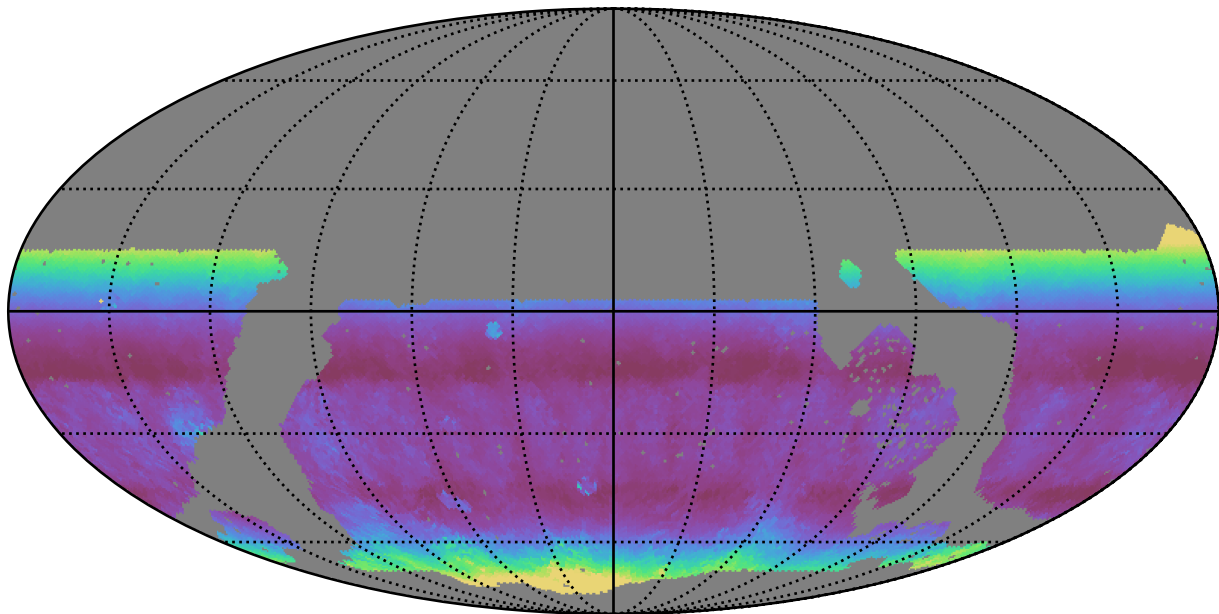
noroll_mjdp270_v3.4_10yrs WFD g band: Median airmass
