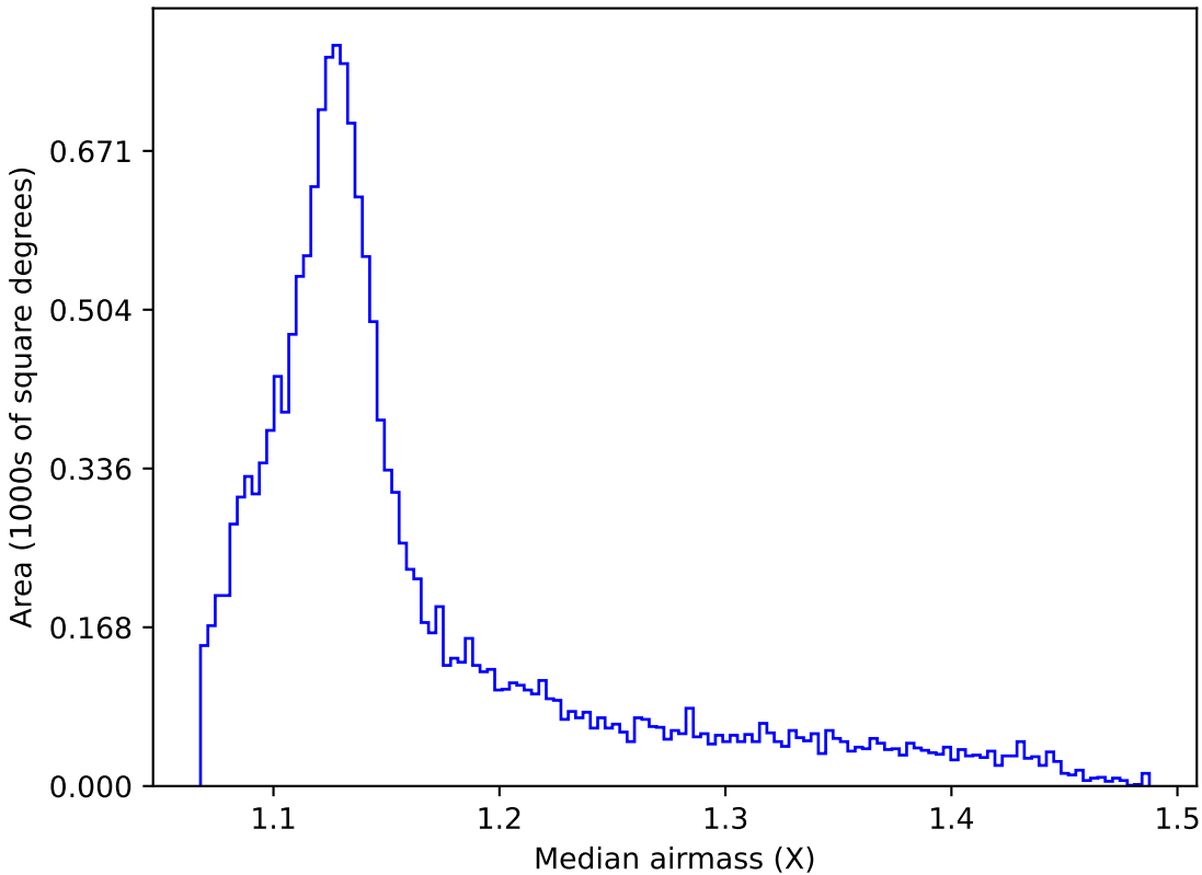
noroll_mjdp270_v3.4_10yrs WFD g band: Median airmass
