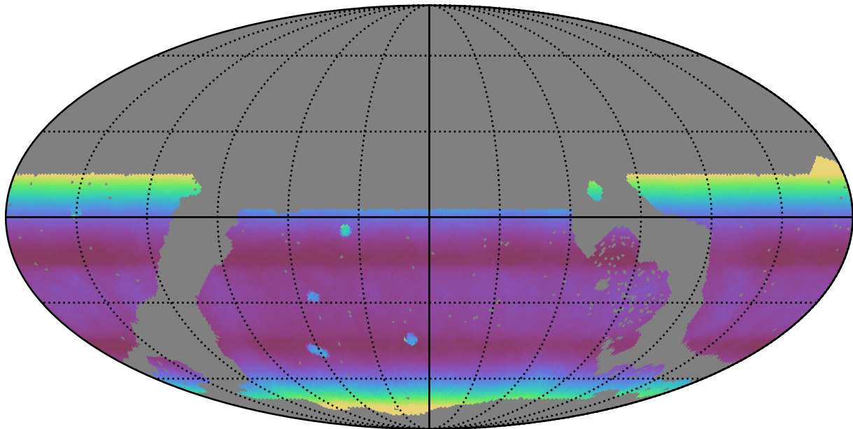
noroll_mjdp270_v3.4_10yrs WFD all bands: Median airmass
