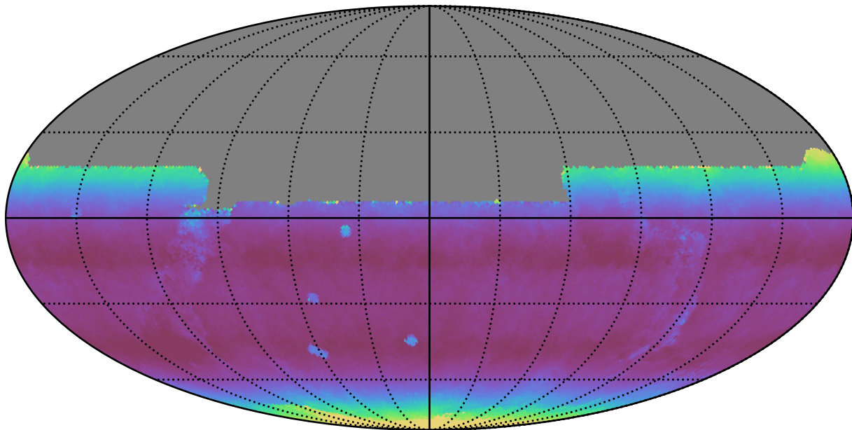
noroll_mjdp270_v3.4_10yrs All sky y band: Median airmass
