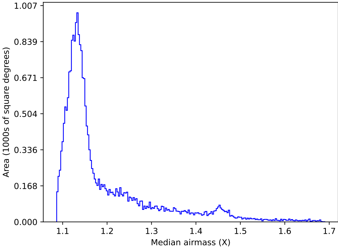
noroll_mjdp270_v3.4_10yrs All sky y band: Median airmass
