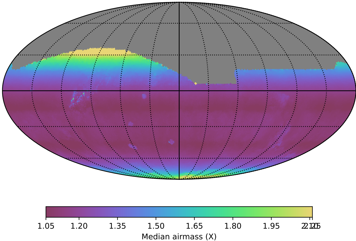
noroll_mjdp270_v3.4_10yrs All sky r band: Median airmass
