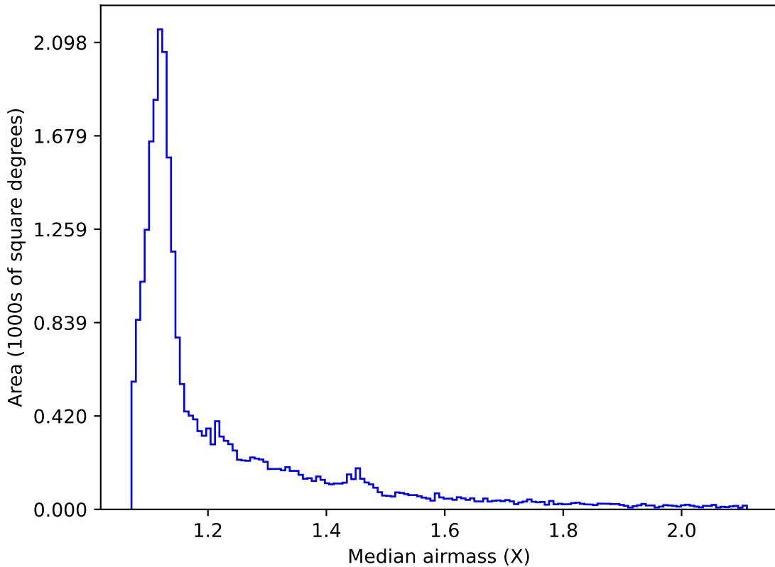
noroll_mjdp270_v3.4_10yrs All sky r band: Median airmass
