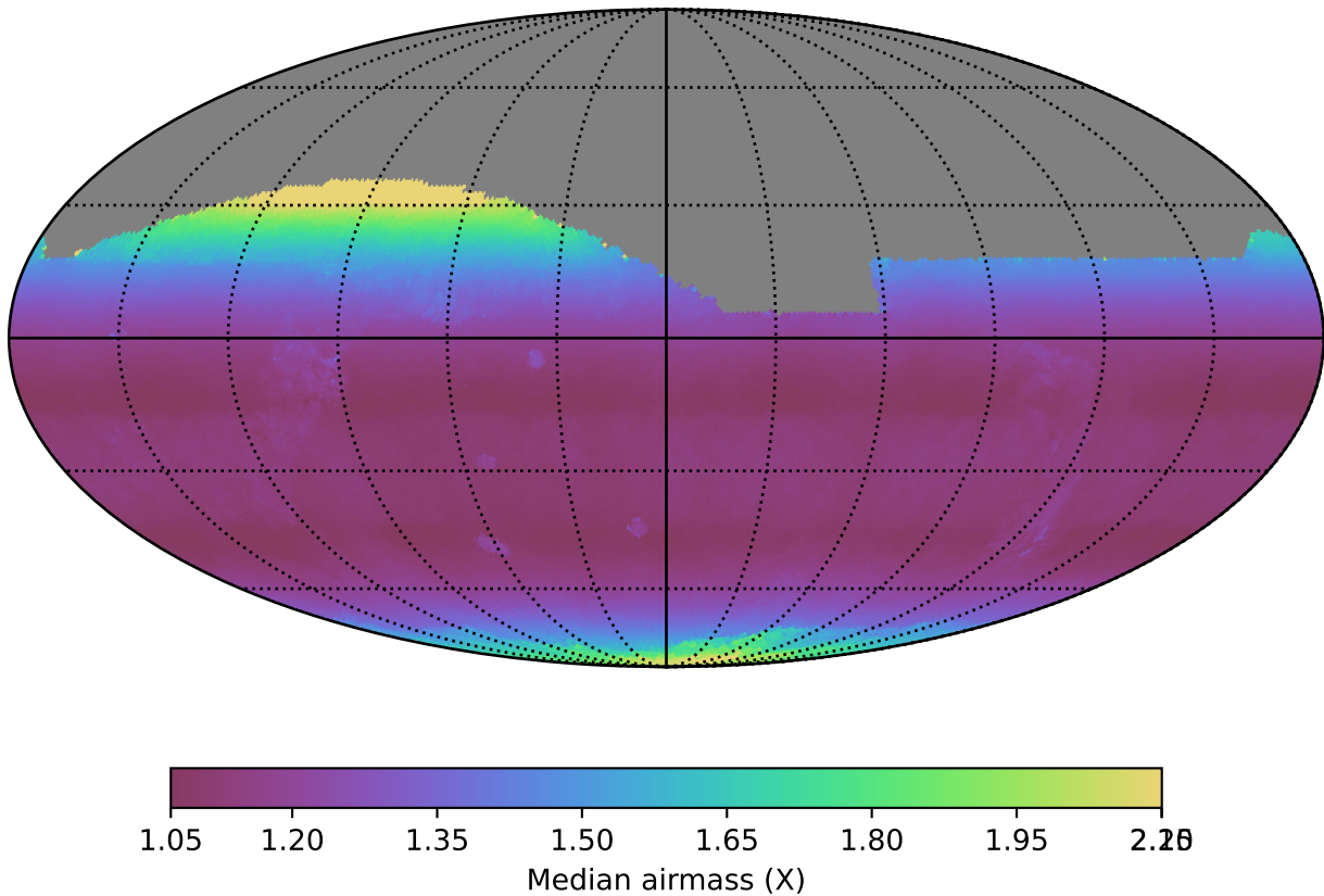
noroll_mjdp270_v3.4_10yrs All sky i band: Median airmass
