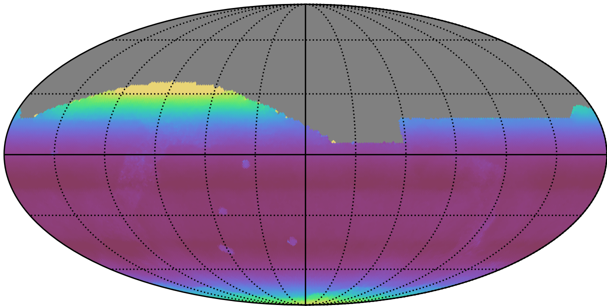
noroll_mjdp270_v3.4_10yrs All sky all bands: Median airmass
