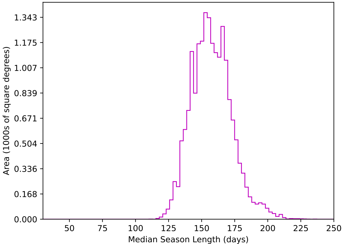
noroll_mjdp270_v3.4_10yrs WFD z band: Median Season Length
