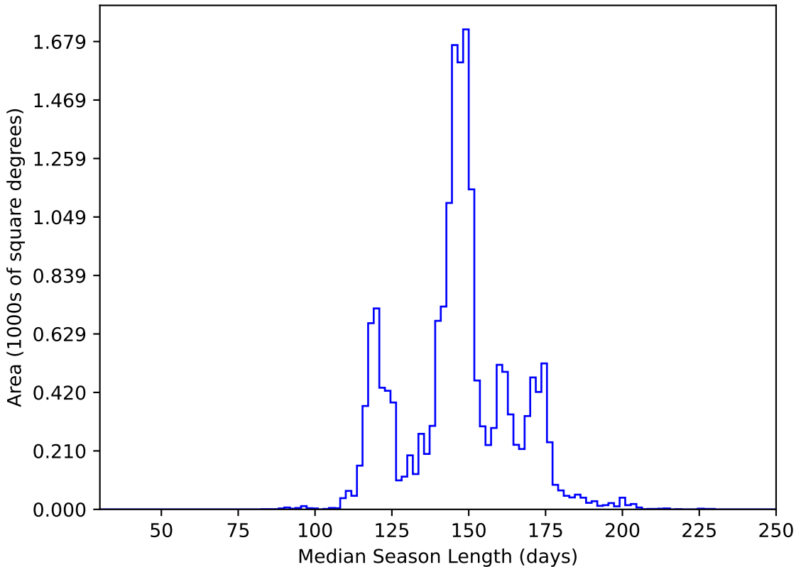
noroll_mjdp270_v3.4_10yrs WFD y band: Median Season Length
