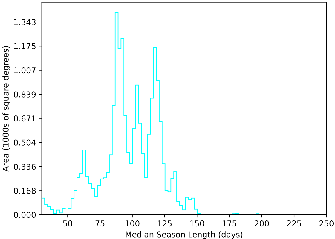
noroll_mjdp270_v3.4_10yrs WFD u band: Median Season Length
