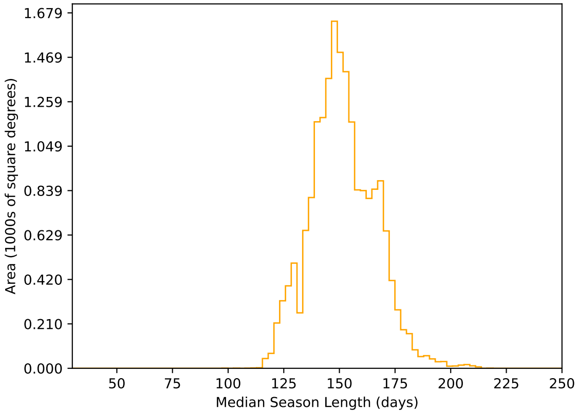
noroll_mjdp270_v3.4_10yrs WFD r band: Median Season Length
