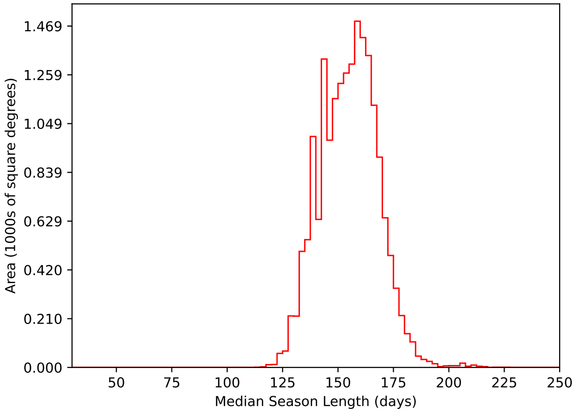
noroll_mjdp270_v3.4_10yrs WFD i band: Median Season Length
