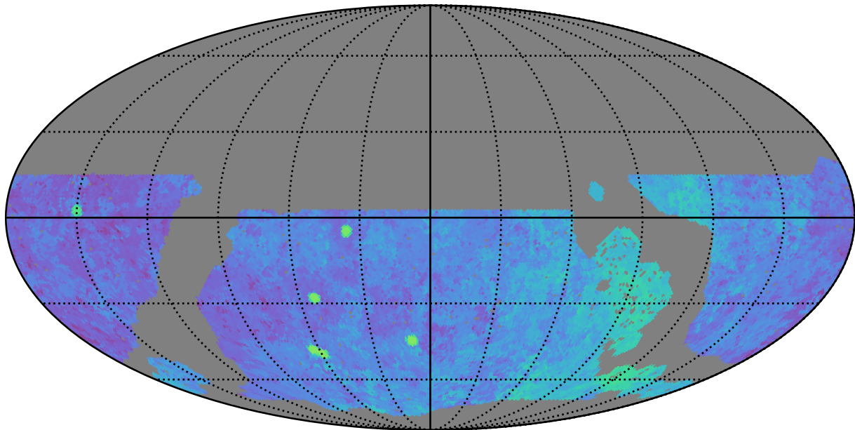
noroll_mjdp270_v3.4_10yrs WFD g band: Median Season Length
