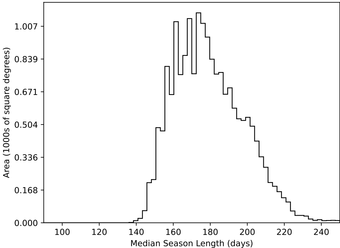
noroll_mjdp270_v3.4_10yrs WFD all bands: Median Season Length
