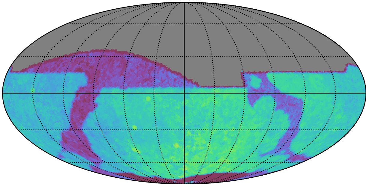
noroll_mjdp270_v3.4_10yrs All sky z band: Median Season Length
